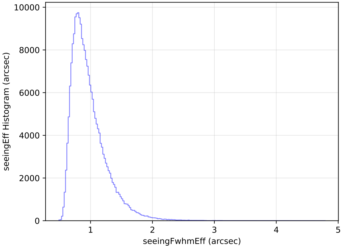
noroll_mjdp270_v3.4_10yrs Yr 1 all bands: seeingEff Histogram
