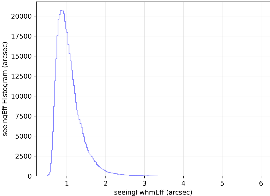
noroll_mjdp270_v3.4_10yrs WFD z band: seeingEff Histogram
