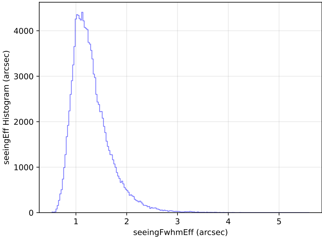
noroll_mjdp270_v3.4_10yrs WFD u band: seeingEff Histogram
