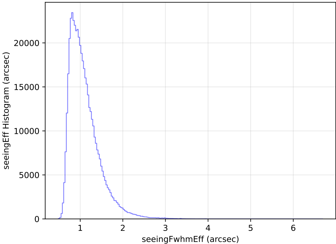
noroll_mjdp270_v3.4_10yrs WFD r band: seeingEff Histogram
