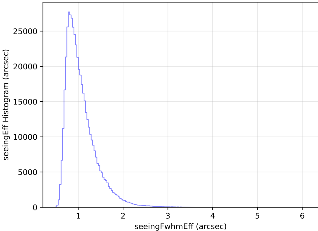
noroll_mjdp270_v3.4_10yrs WFD i band: seeingEff Histogram
