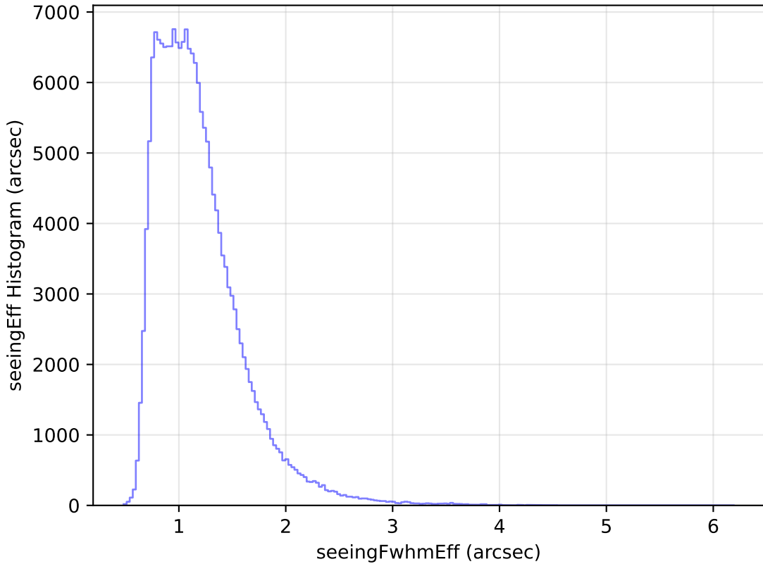
noroll_mjdp270_v3.4_10yrs WFD g band: seeingEff Histogram
