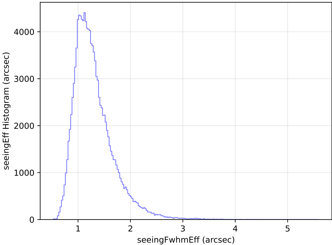
noroll_mjdp270_v3.4_10yrs All sky u band: seeingEff Histogram
