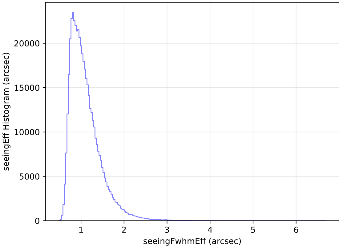
noroll_mjdp270_v3.4_10yrs All sky r band: seeingEff Histogram
