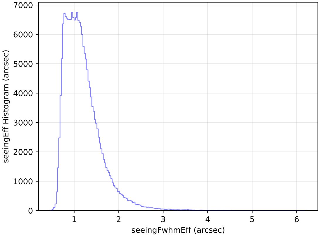
noroll_mjdp270_v3.4_10yrs All sky g band: seeingEff Histogram
