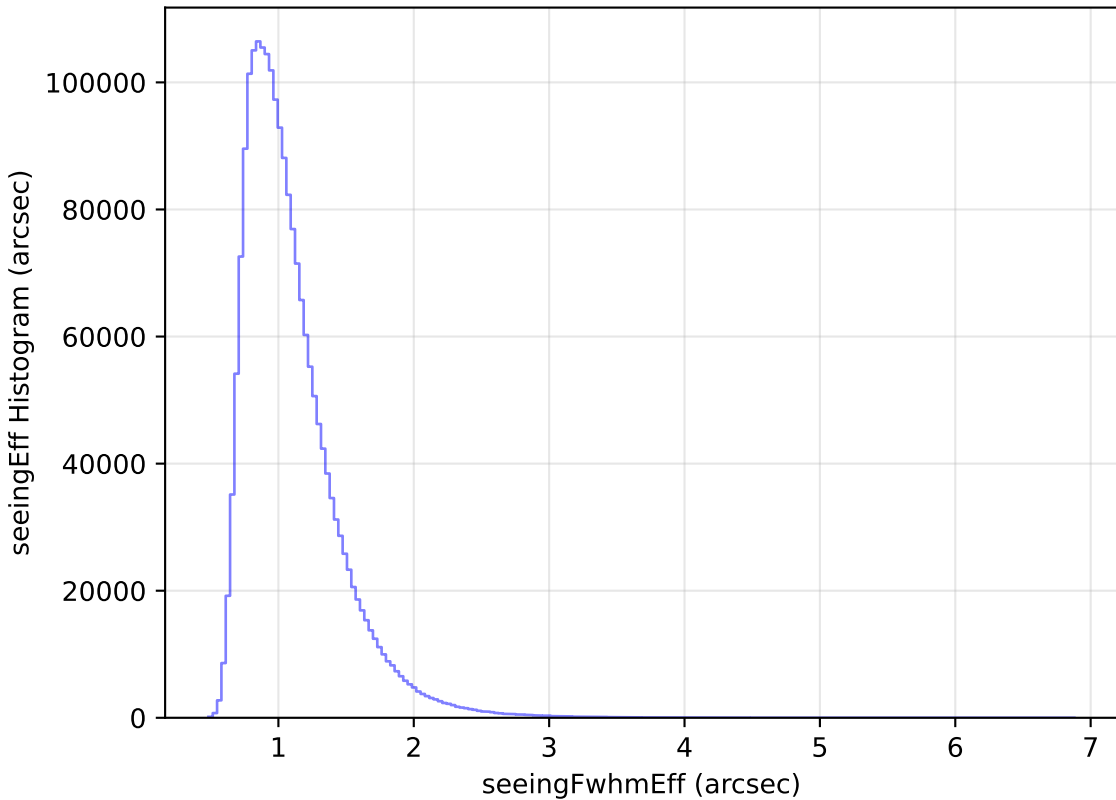
noroll_mjdp270_v3.4_10yrs All sky all bands: seeingEff Histogram
