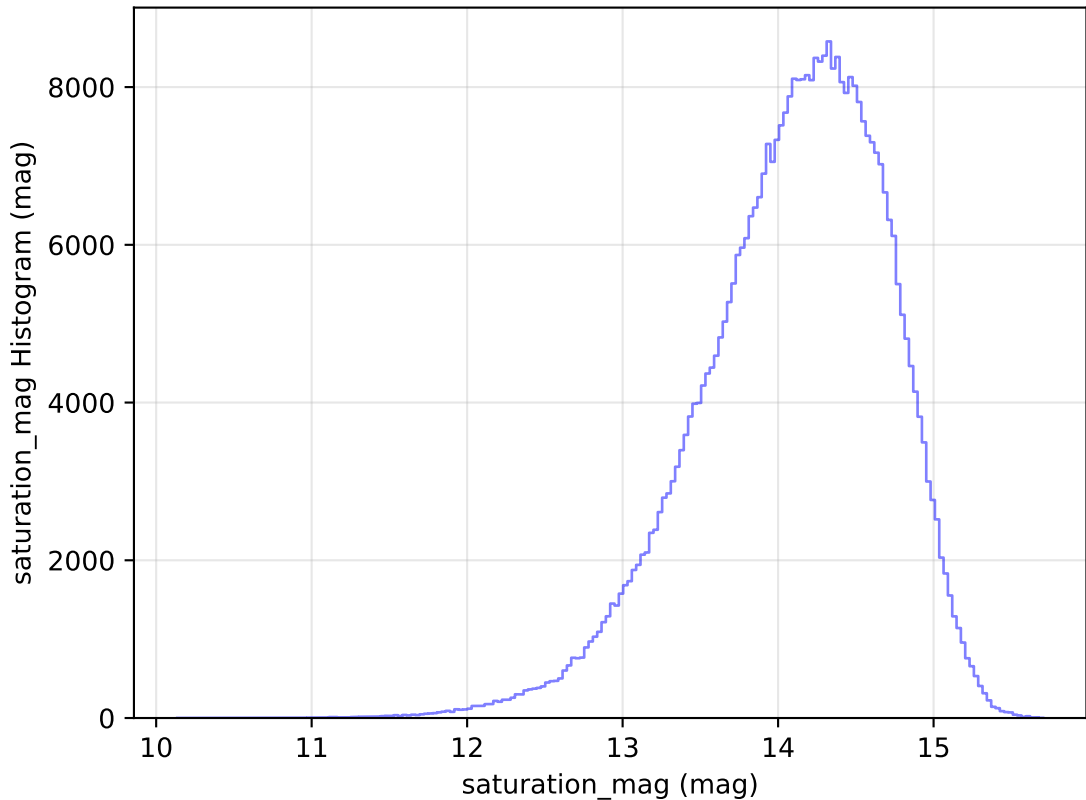
noroll_mjdp270_v3.4_10yrs WFD z band: saturation_mag Histogram
