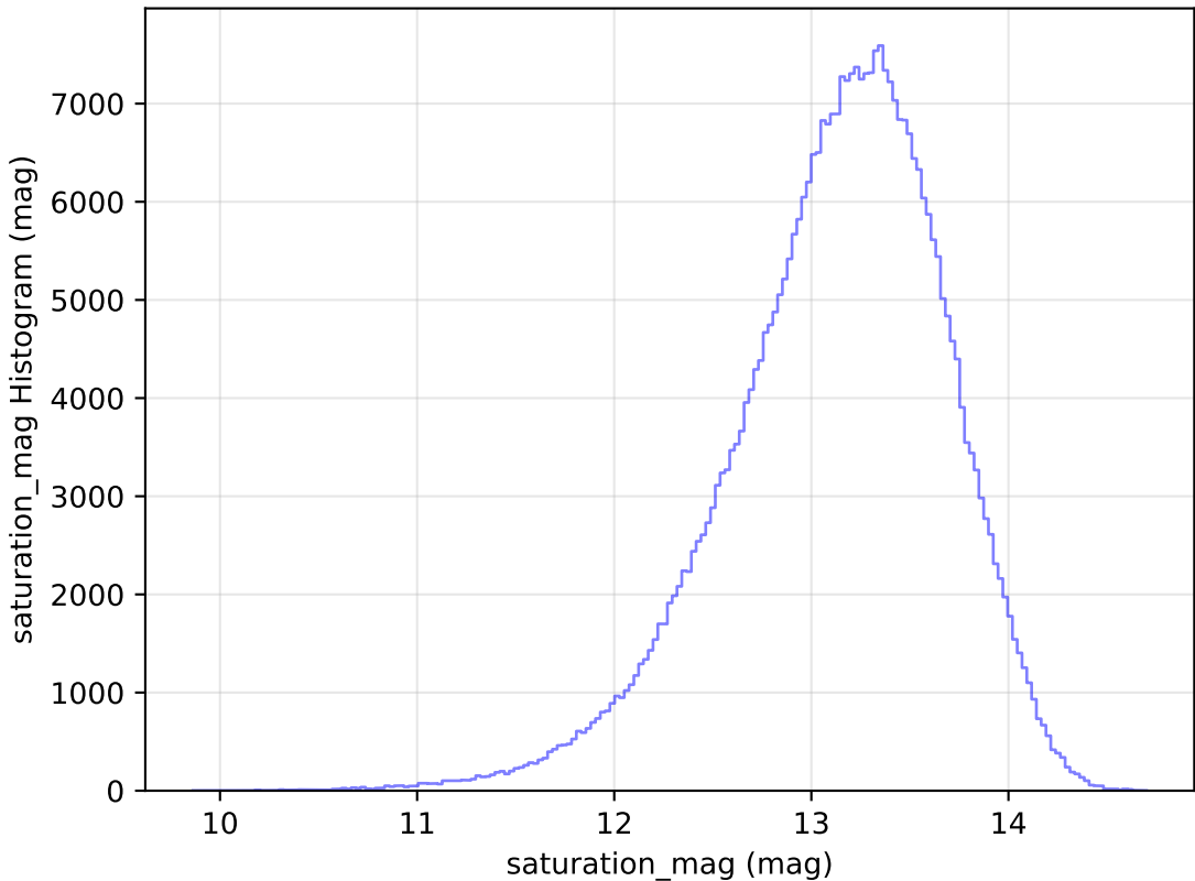
noroll_mjdp270_v3.4_10yrs WFD y band: saturation_mag Histogram
