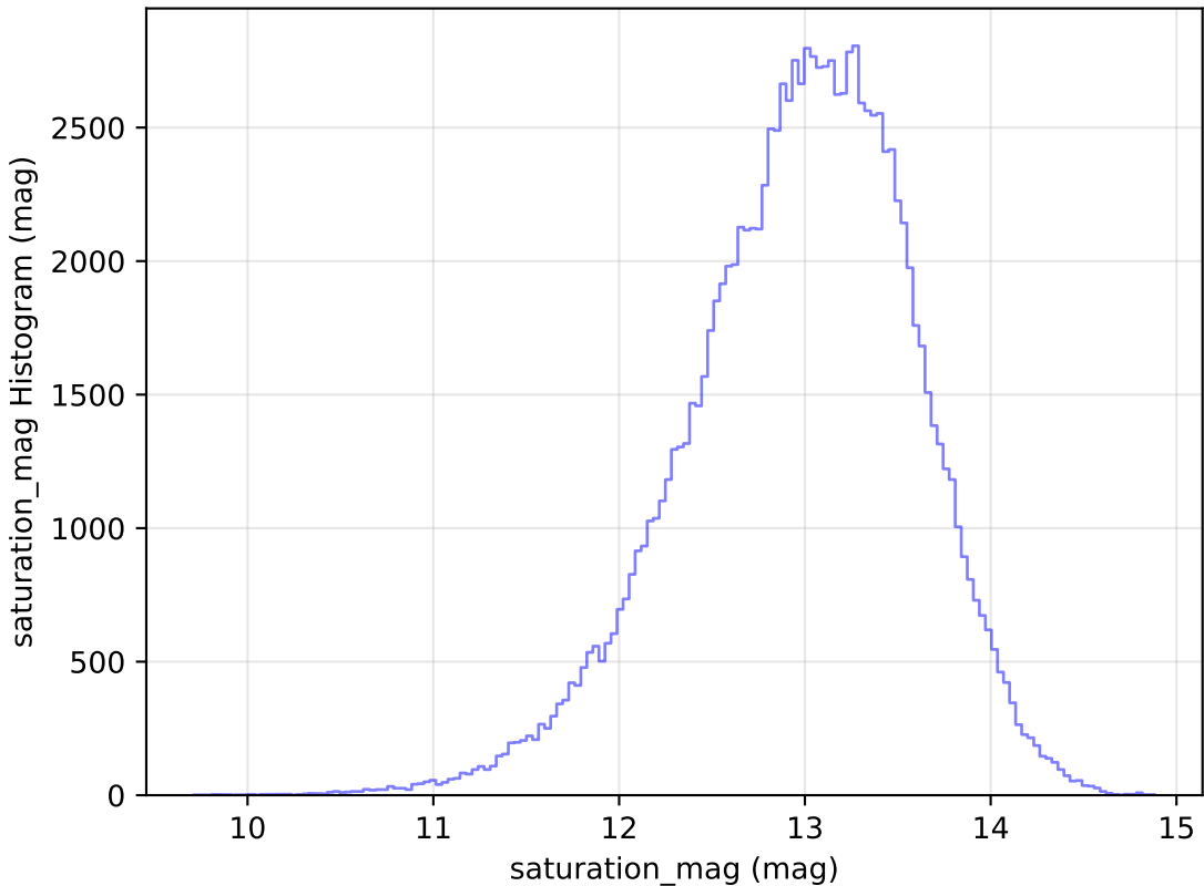
noroll_mjdp270_v3.4_10yrs WFD u band: saturation_mag Histogram
