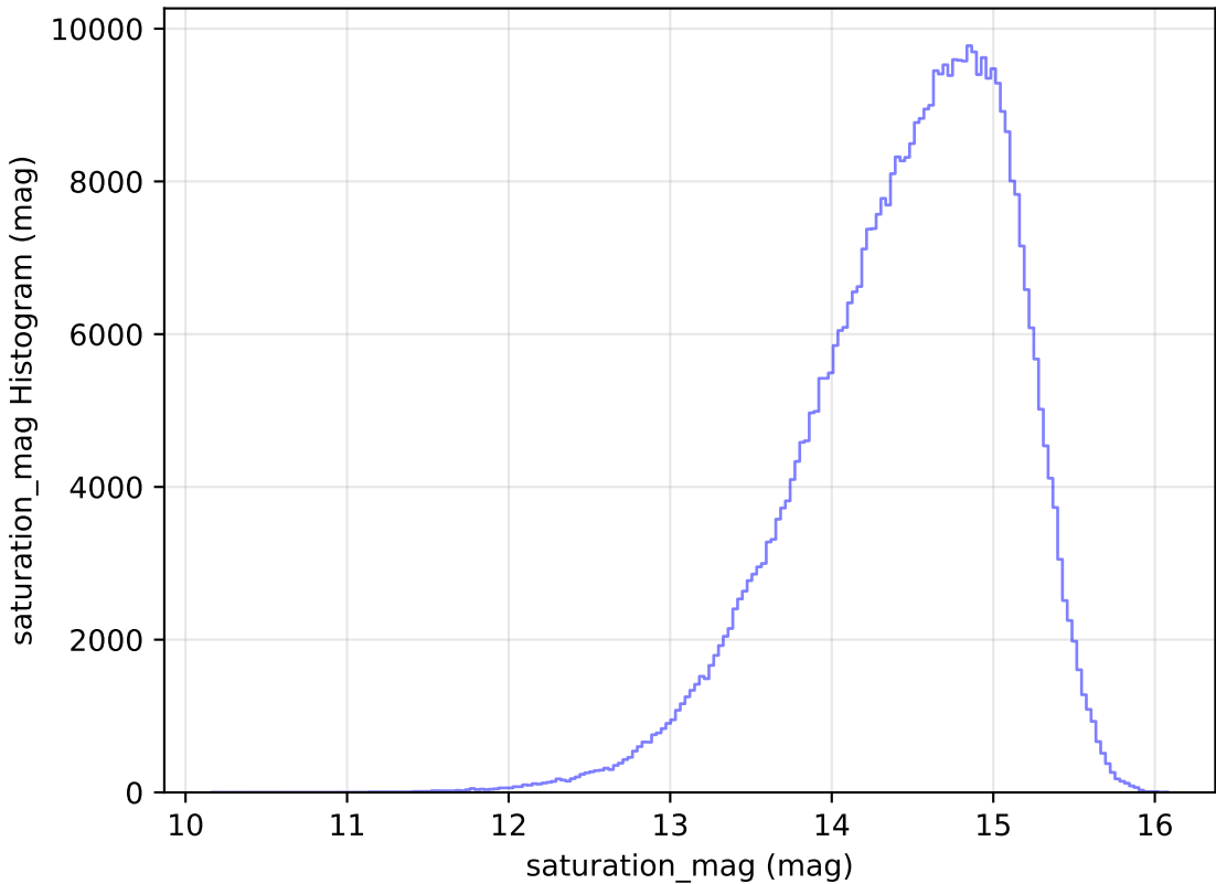
noroll_mjdp270_v3.4_10yrs WFD i band: saturation_mag Histogram
