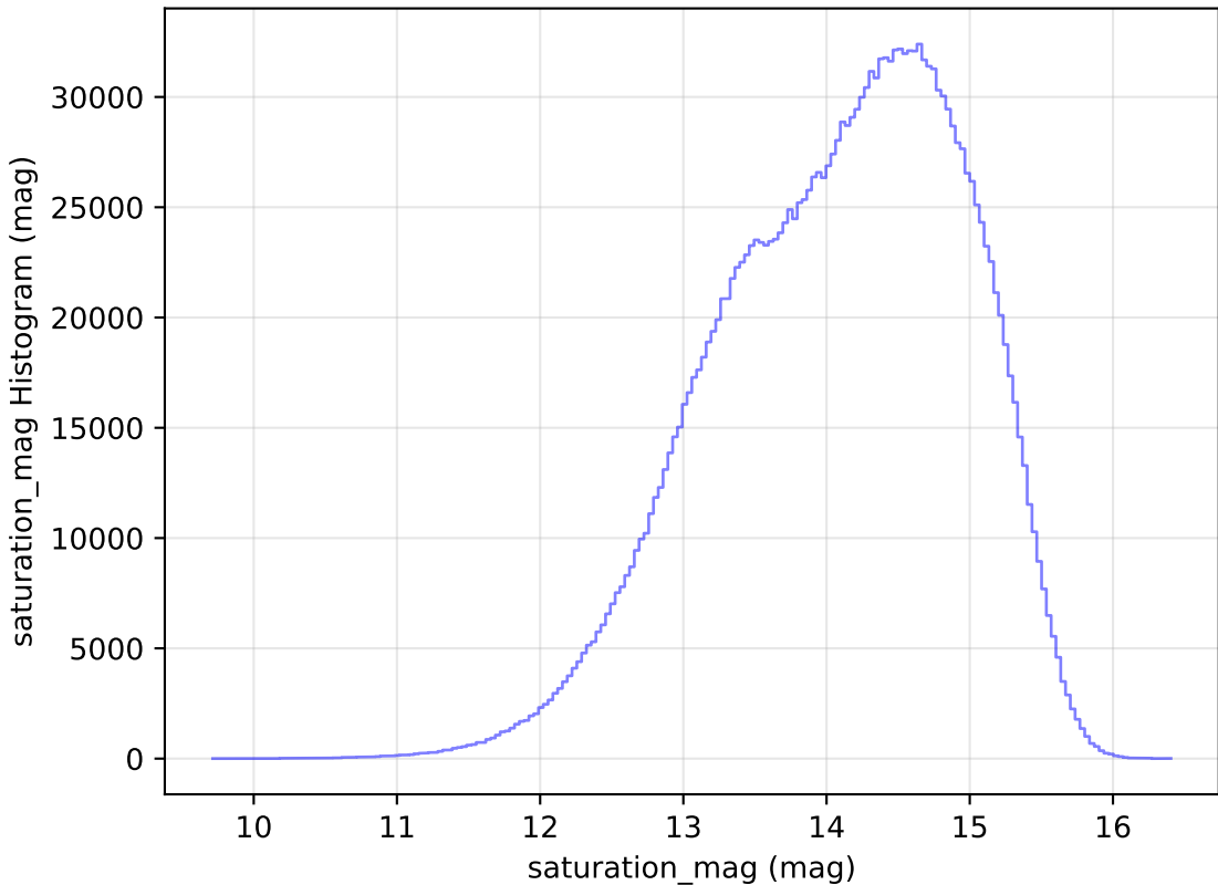
noroll_mjdp270_v3.4_10yrs WFD all bands: saturation_mag Histogram
