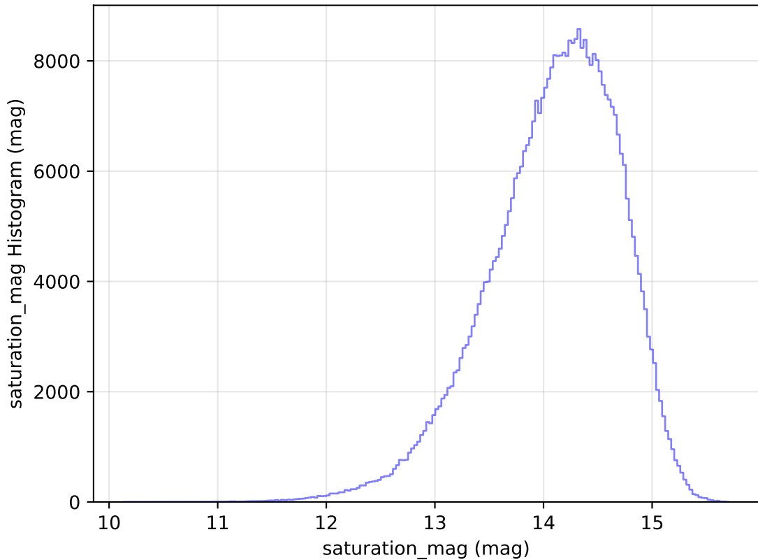
noroll_mjdp270_v3.4_10yrs All sky z band: saturation_mag Histogram
