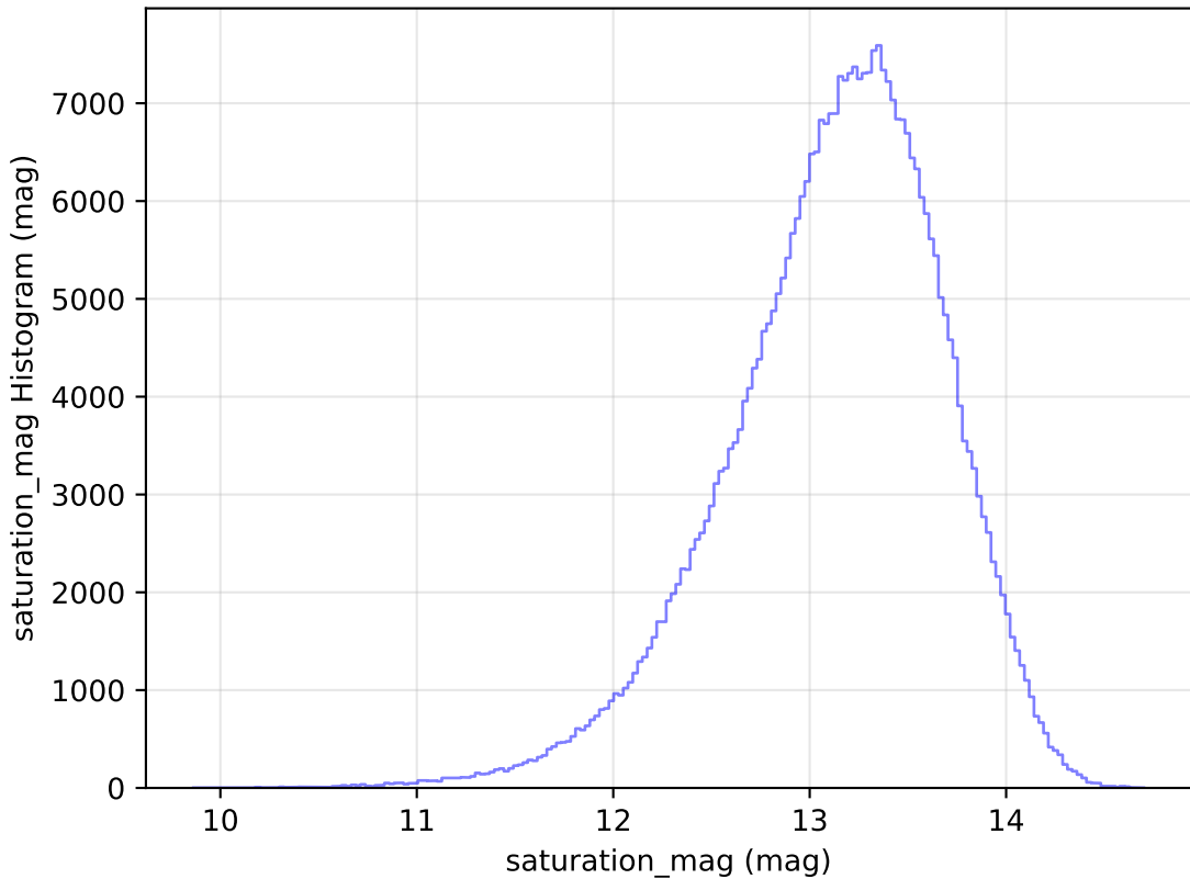
noroll_mjdp270_v3.4_10yrs All sky y band: saturation_mag Histogram
