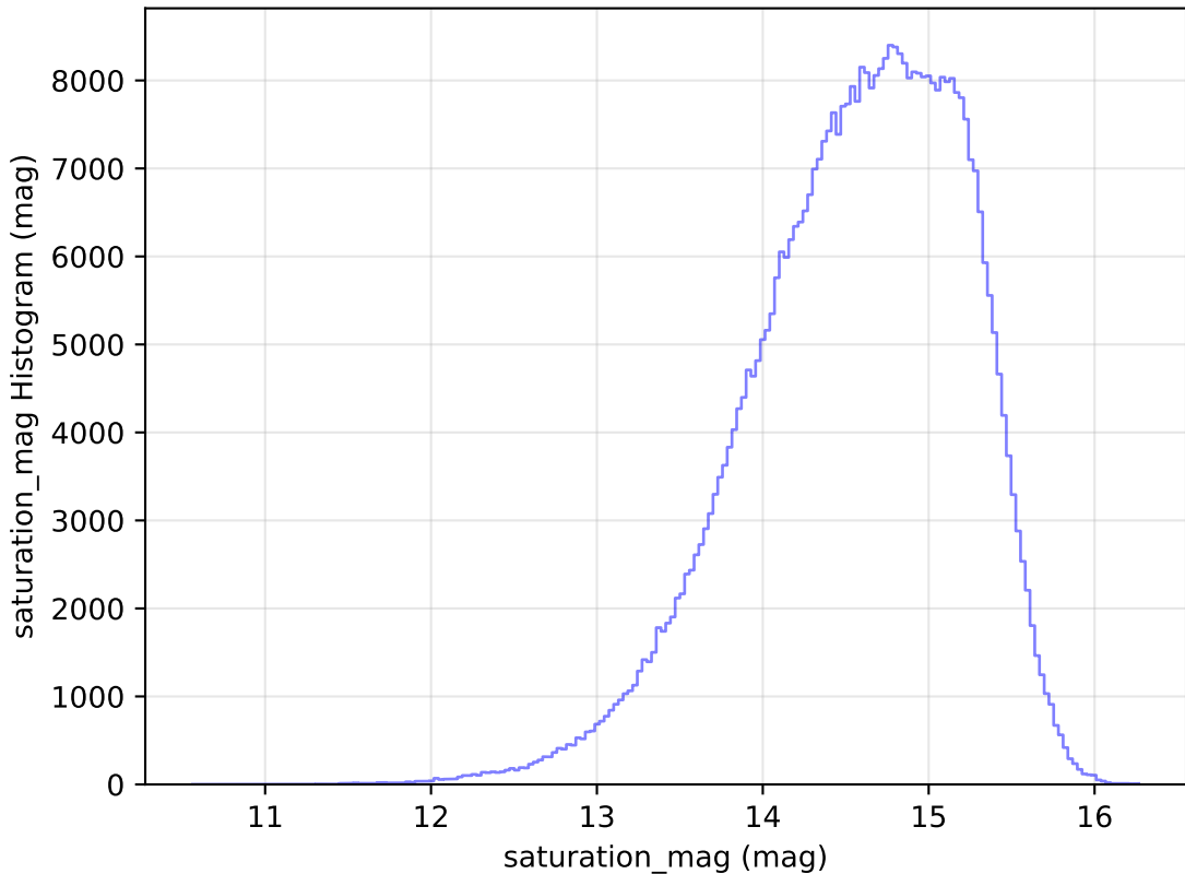
noroll_mjdp270_v3.4_10yrs All sky r band: saturation_mag Histogram
