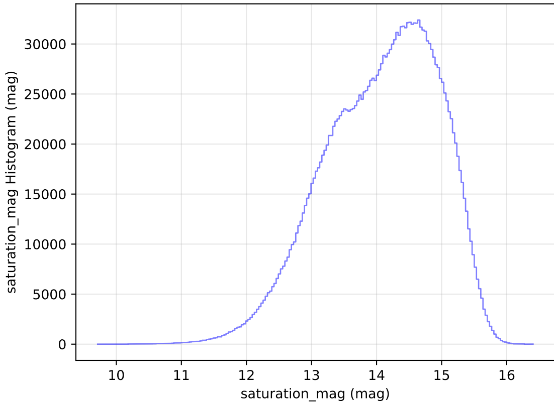
noroll_mjdp270_v3.4_10yrs All sky all bands: saturation_mag Histogram
