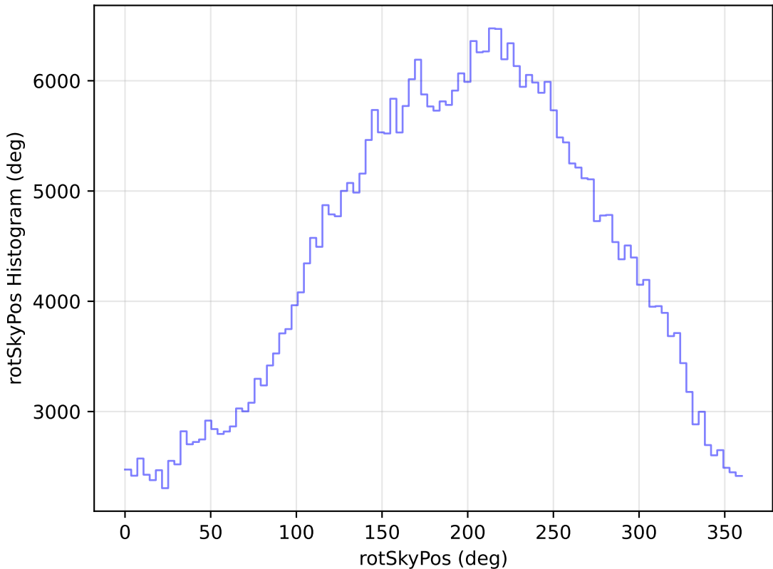
noroll_mjdp270_v3.4_10yrs WFD z band: rotSkyPos Histogram
