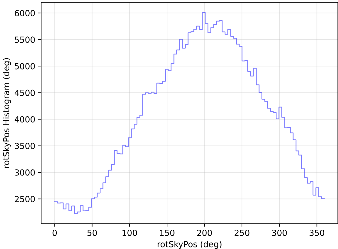
noroll_mjdp270_v3.4_10yrs WFD y band: rotSkyPos Histogram
