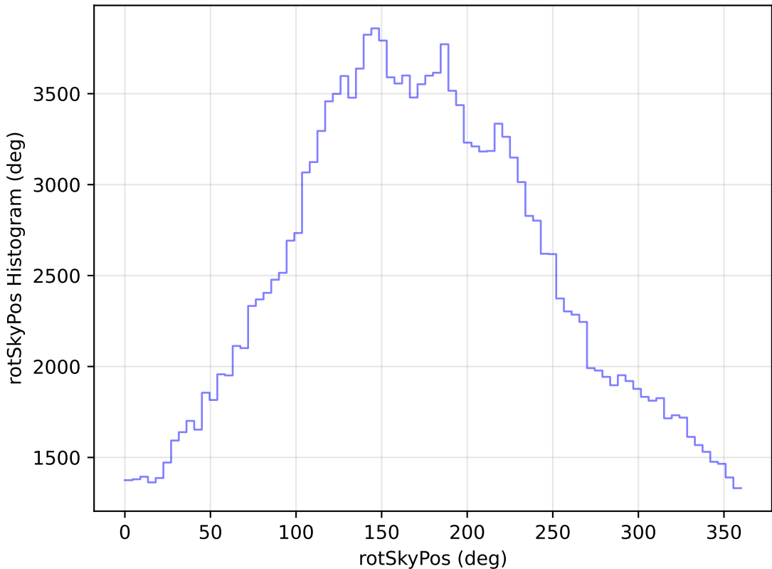
noroll_mjdp270_v3.4_10yrs WFD g band: rotSkyPos Histogram
