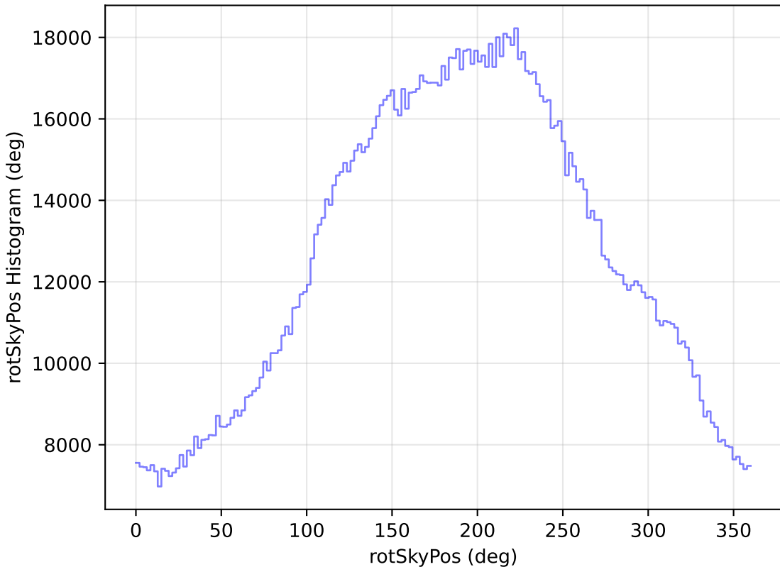
noroll_mjdp270_v3.4_10yrs WFD all bands: rotSkyPos Histogram
