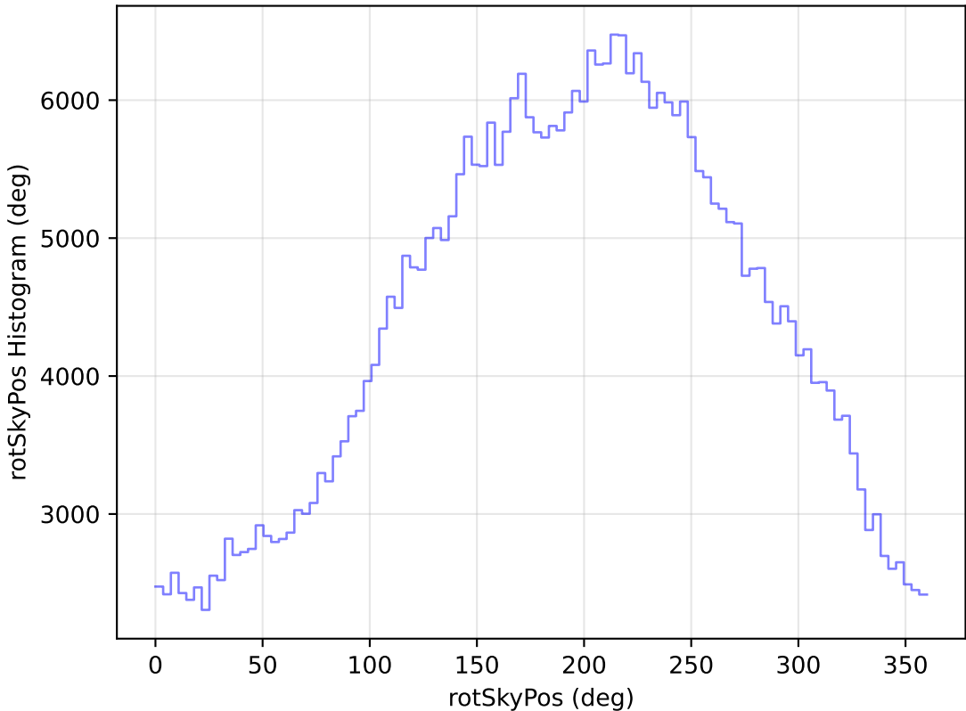
noroll_mjdp270_v3.4_10yrs All sky z band: rotSkyPos Histogram
