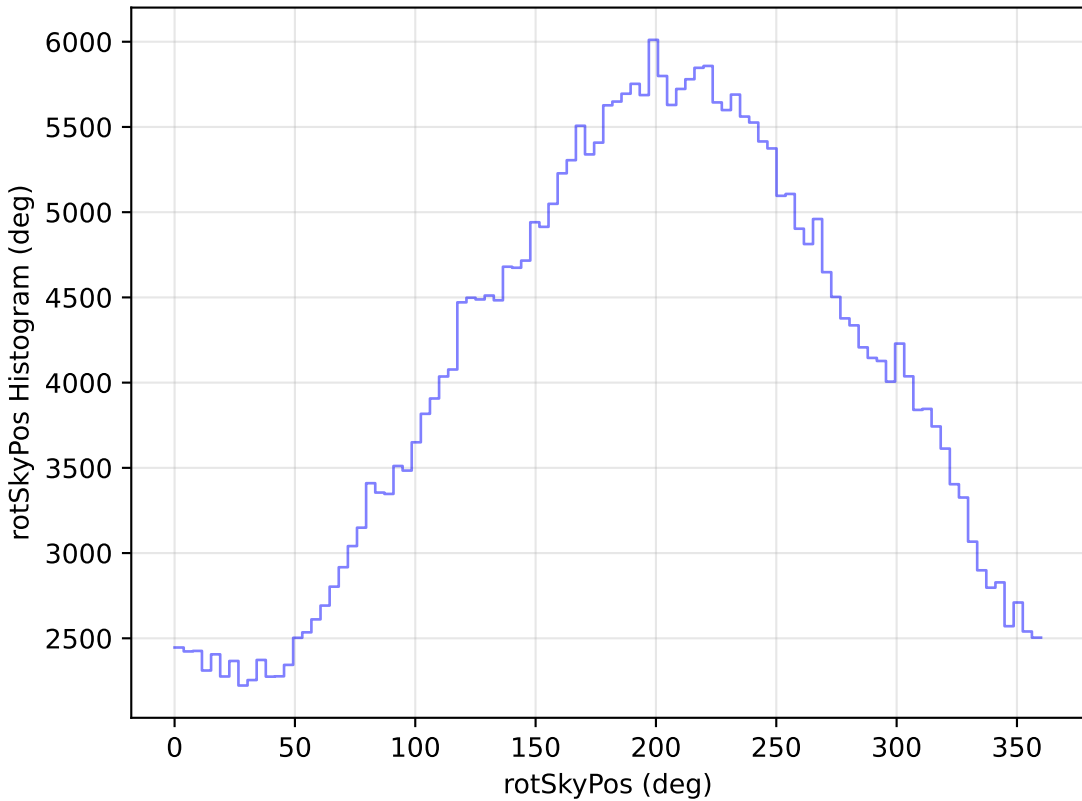
noroll_mjdp270_v3.4_10yrs All sky y band: rotSkyPos Histogram
