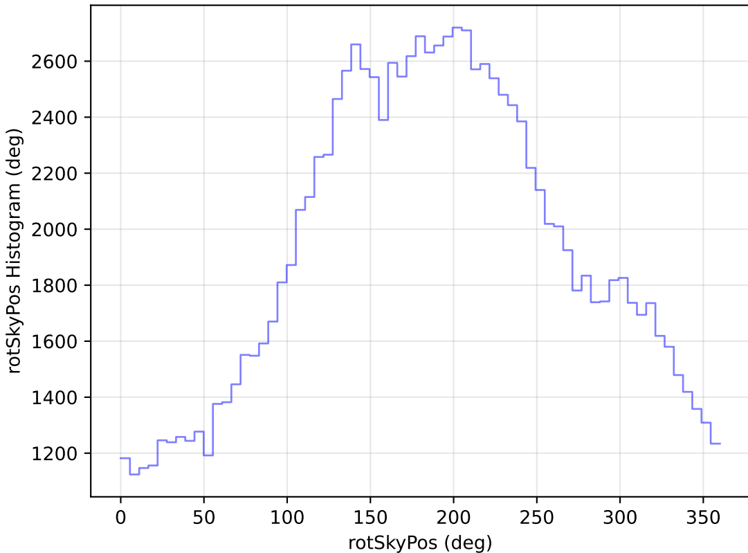
noroll_mjdp270_v3.4_10yrs All sky u band: rotSkyPos Histogram
