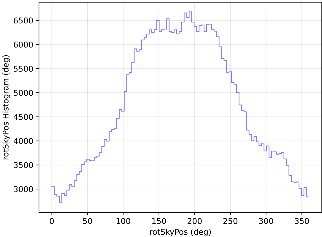
noroll_mjdp270_v3.4_10yrs All sky r band: rotSkyPos Histogram
