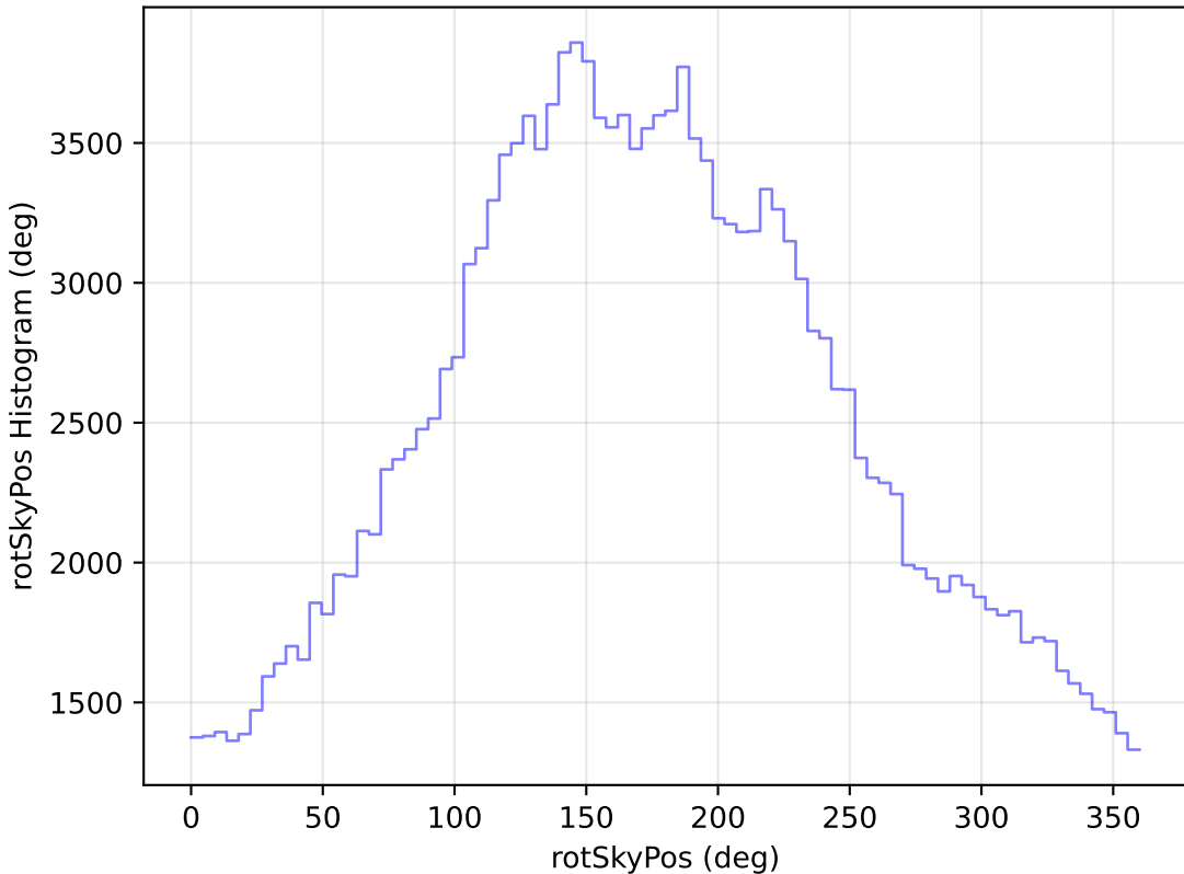
noroll_mjdp270_v3.4_10yrs All sky g band: rotSkyPos Histogram
