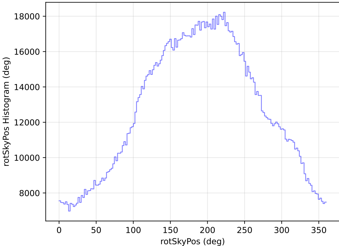
noroll_mjdp270_v3.4_10yrs All sky all bands: rotSkyPos Histogram
