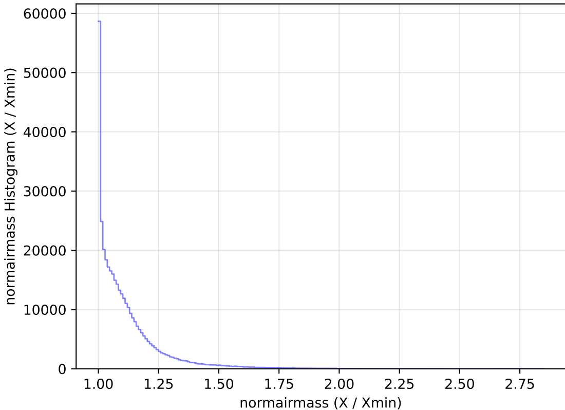
noroll_mjdp270_v3.4_10yrs WFD y band: normairmass Histogram
