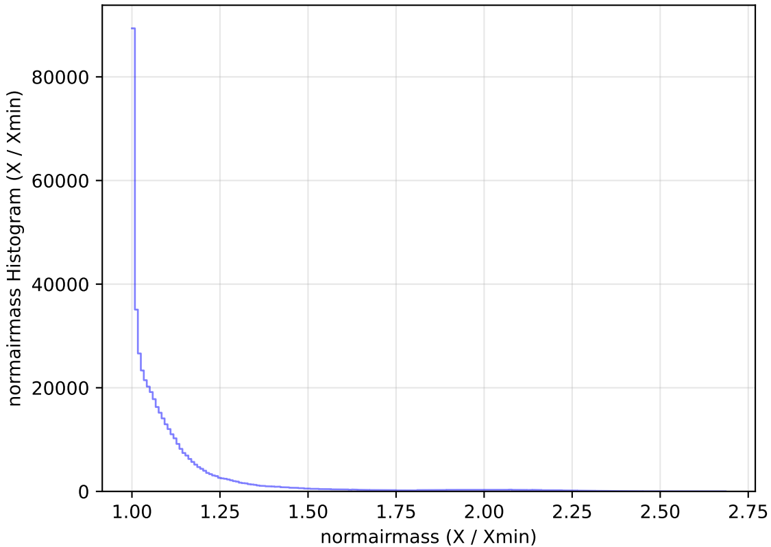
noroll_mjdp270_v3.4_10yrs WFD r band: normairmass Histogram
