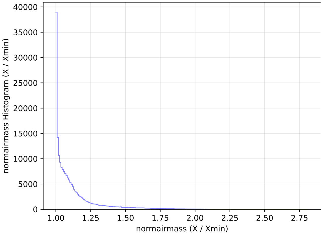
noroll_mjdp270_v3.4_10yrs WFD g band: normairmass Histogram
