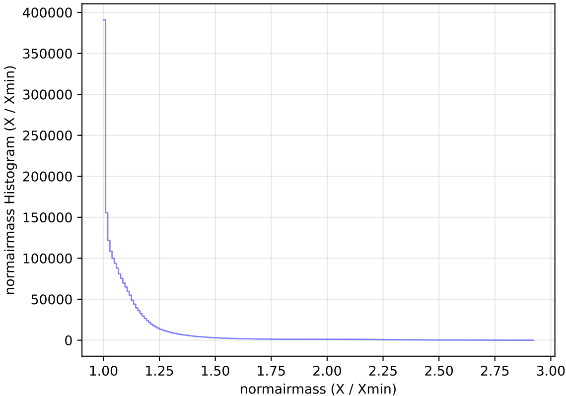
noroll_mjdp270_v3.4_10yrs WFD all bands: normairmass Histogram
