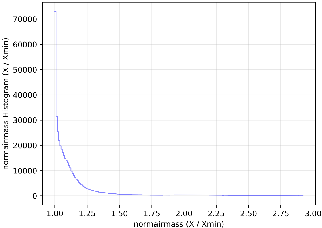
noroll_mjdp270_v3.4_10yrs All sky z band: normairmass Histogram
