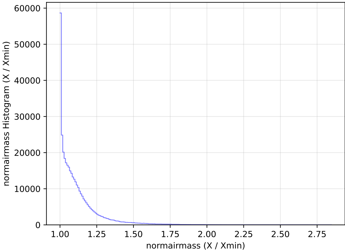
noroll_mjdp270_v3.4_10yrs All sky y band: normairmass Histogram
