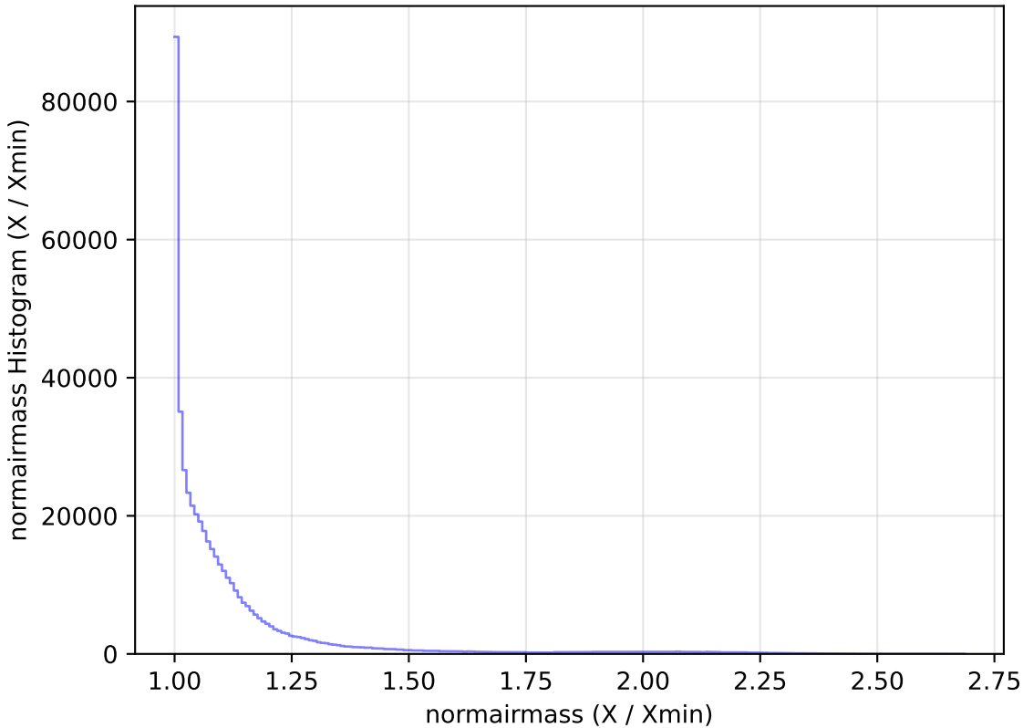
noroll_mjdp270_v3.4_10yrs All sky r band: normairmass Histogram
