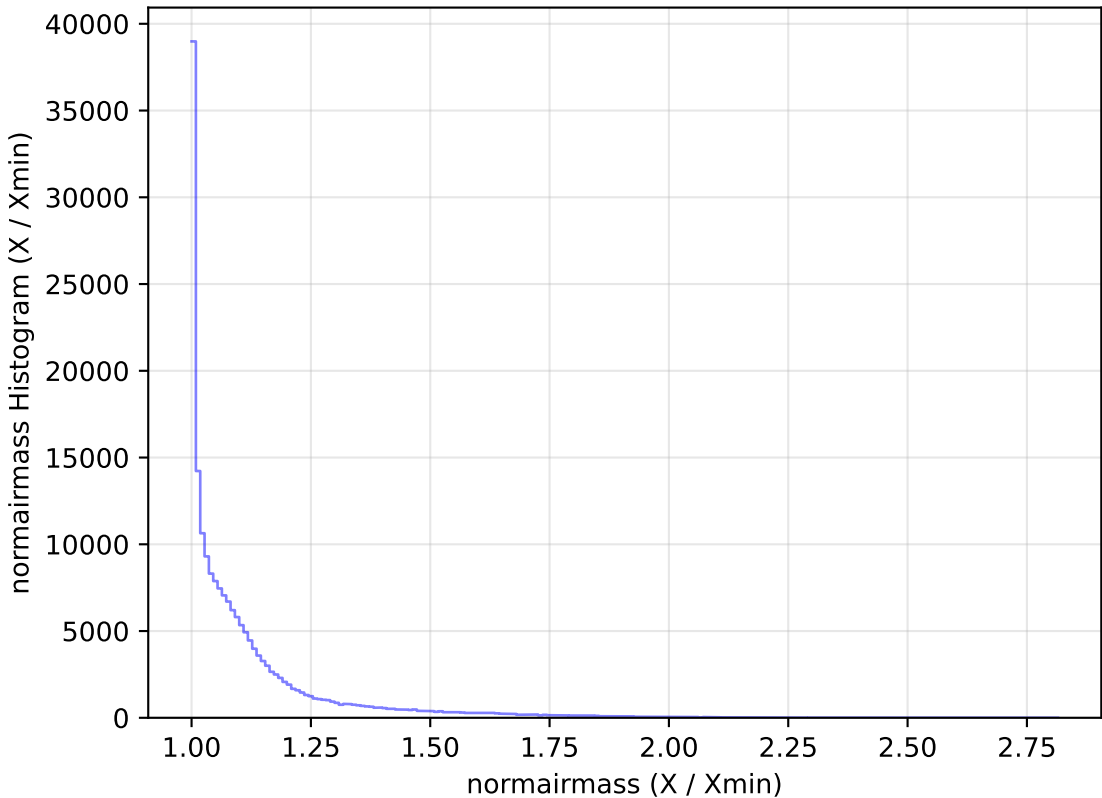
noroll_mjdp270_v3.4_10yrs All sky g band: normairmass Histogram
