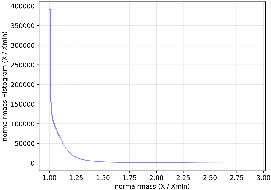
noroll_mjdp270_v3.4_10yrs All sky all bands: normairmass Histogram
