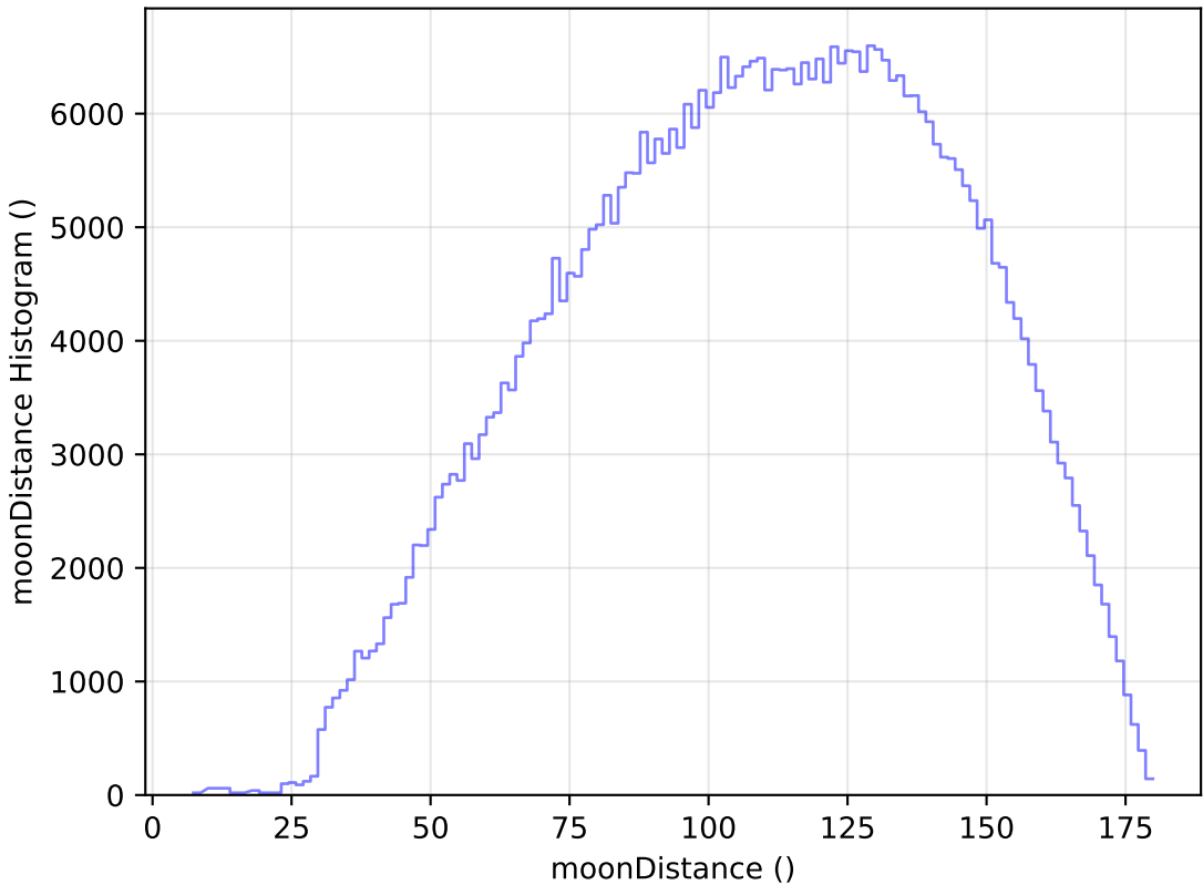
noroll_mjdp270_v3.4_10yrs WFD r band: moonDistance Histogram
