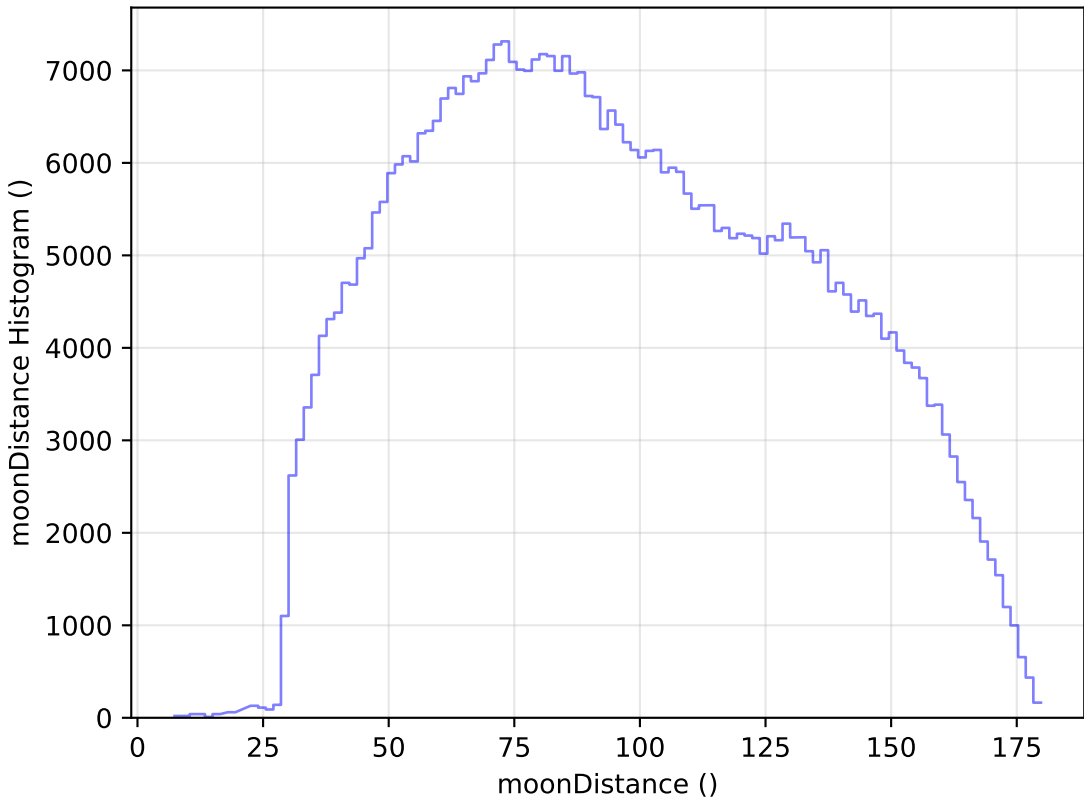
noroll_mjdp270_v3.4_10yrs WFD i band: moonDistance Histogram
