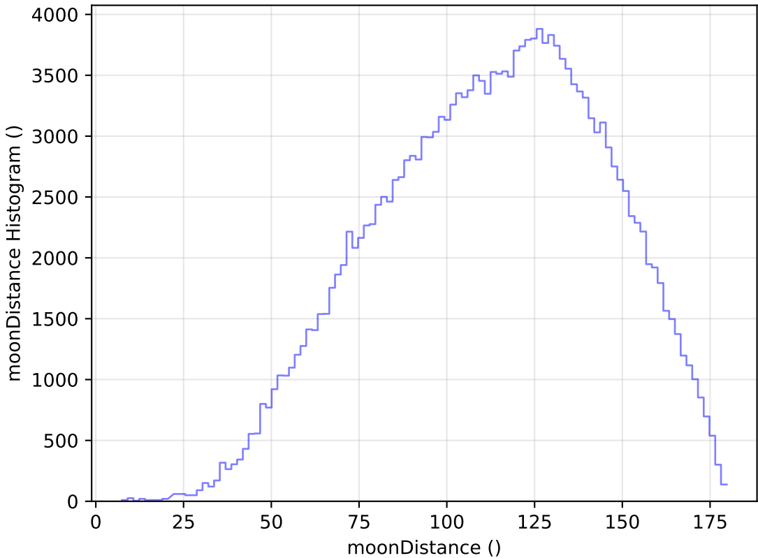
noroll_mjdp270_v3.4_10yrs WFD g band: moonDistance Histogram
