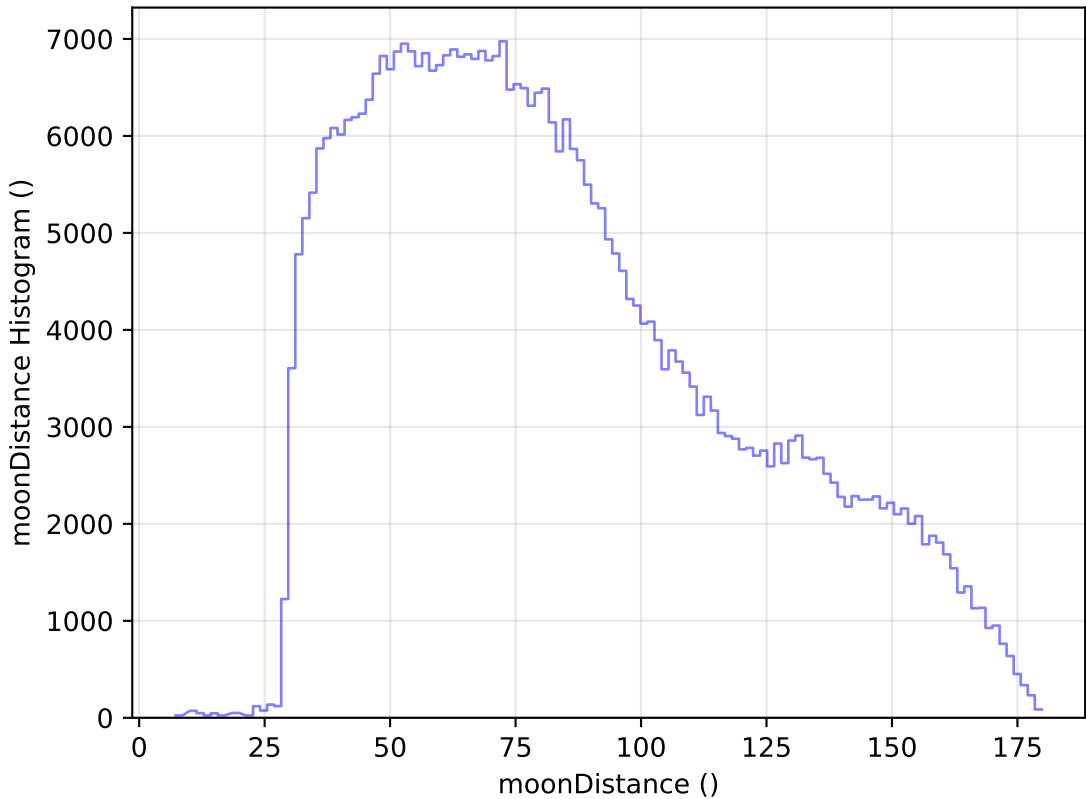
noroll_mjdp270_v3.4_10yrs All sky z band: moonDistance Histogram
