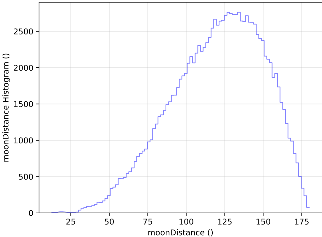
noroll_mjdp270_v3.4_10yrs All sky u band: moonDistance Histogram
