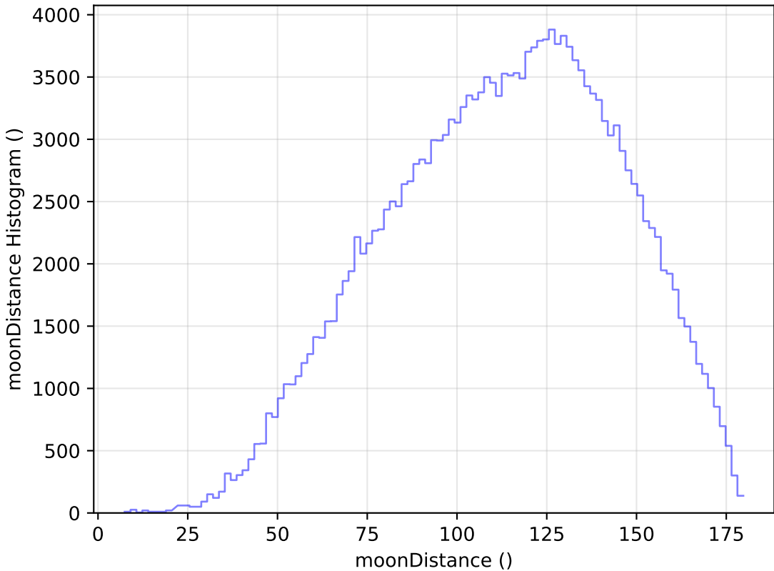
noroll_mjdp270_v3.4_10yrs All sky g band: moonDistance Histogram
