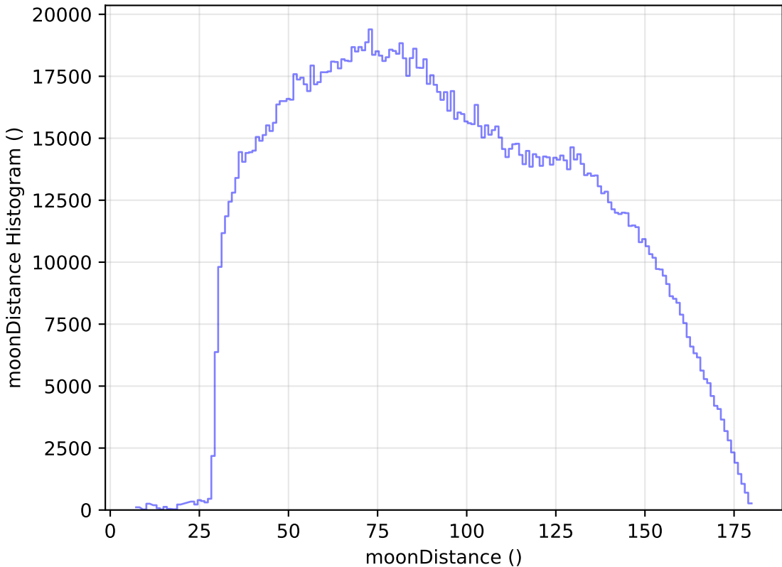
noroll_mjdp270_v3.4_10yrs All sky all bands: moonDistance Histogram
