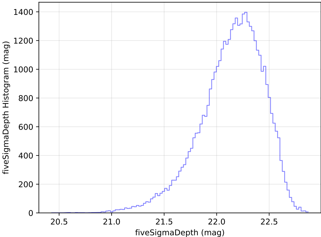
noroll_mjdp270_v3.4_10yrs Yr 1 y band: fiveSigmaDepth Histogram
