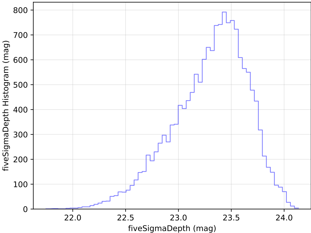
noroll_mjdp270_v3.4_10yrs Yr 1 u band: fiveSigmaDepth Histogram
