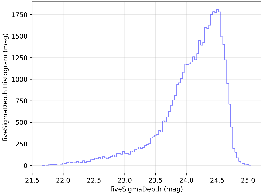
noroll_mjdp270_v3.4_10yrs Yr 1 r band: fiveSigmaDepth Histogram
