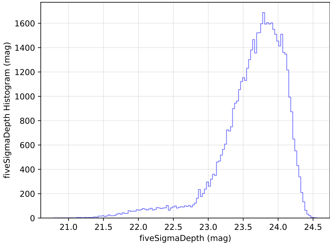
noroll_mjdp270_v3.4_10yrs Yr 1 i band: fiveSigmaDepth Histogram
