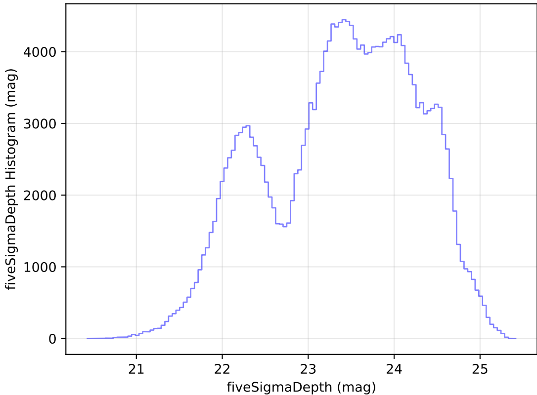
noroll_mjdp270_v3.4_10yrs Yr 1 all bands: fiveSigmaDepth Histogram
